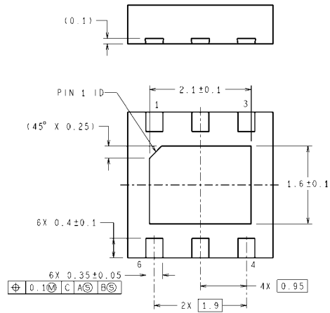
LLP, 6 Lead, Package (SOT23 Land) NS Package Number SDE06A
